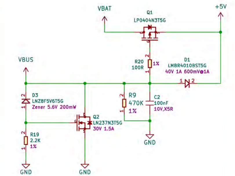
BAT Charger
